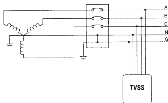
Fig. 2: 3-Phase, 4-Wire + Ground
